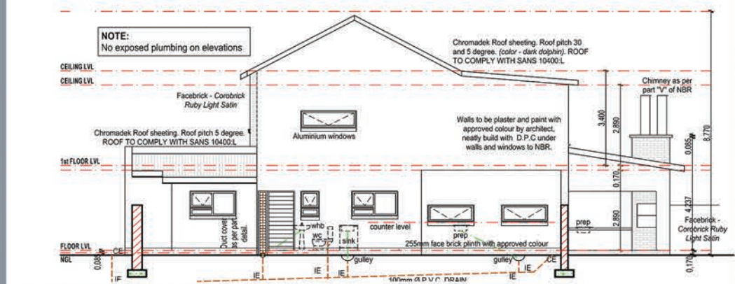
EAST ELEVATION
