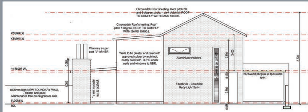
WEST ELEVATION
