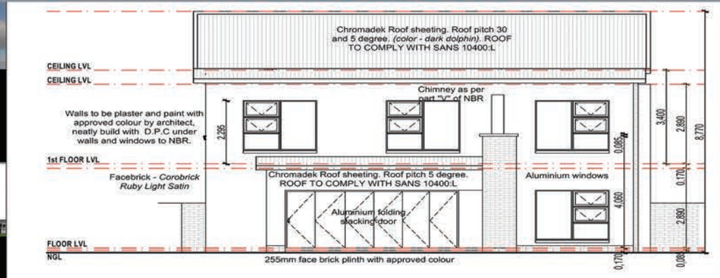
NORTH ELEVATION
