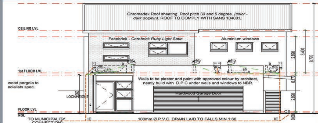
SOUTH ELEVATION
